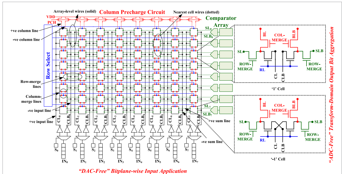
Figure 22. Compute-in-SRAM designs exploit analog computations to exploit ‘physics for computing,’ however suffer due to the use of many digital-to-analog converters (DAC) and analog-to-digital converters (ADC) for each memory array which limits their scalability and energy efficiency. Novel implementation methods have exploited co-design methods such as transform-domain neural network operations to overcome these limitations [152]. The co-designed approach has achieved orders of magnitude more energy efficiency and significant scalability over the traditional compute-in-memory implementation.
